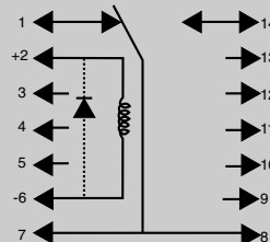
1 Form C
