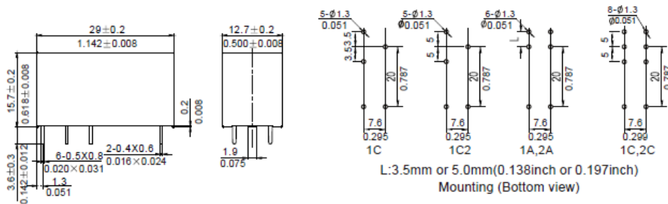
Dimension
