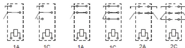
Wiring diagram (Bottom view)
